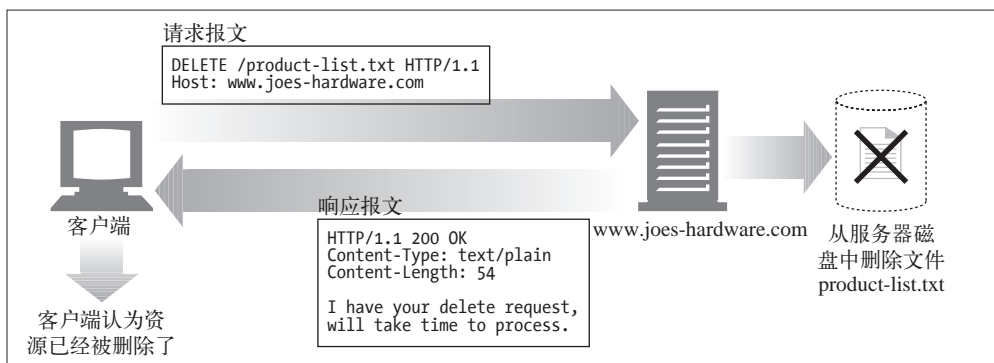
图 3-13 DELETE 示例
