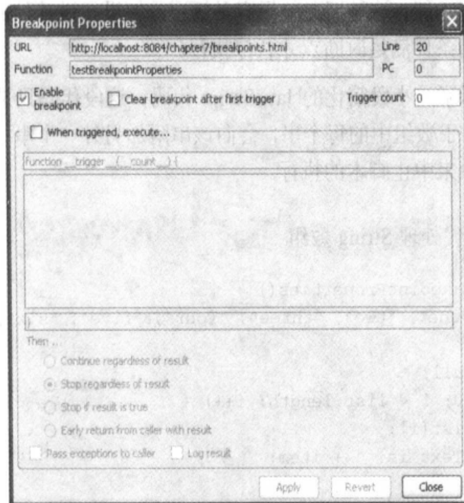
图 7-20 Breakpoint Properties 窗口的默认外观
