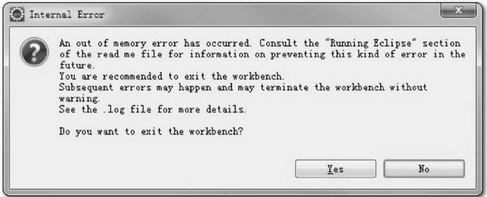
图 5-5 Eclipse OutOfMemoryError
